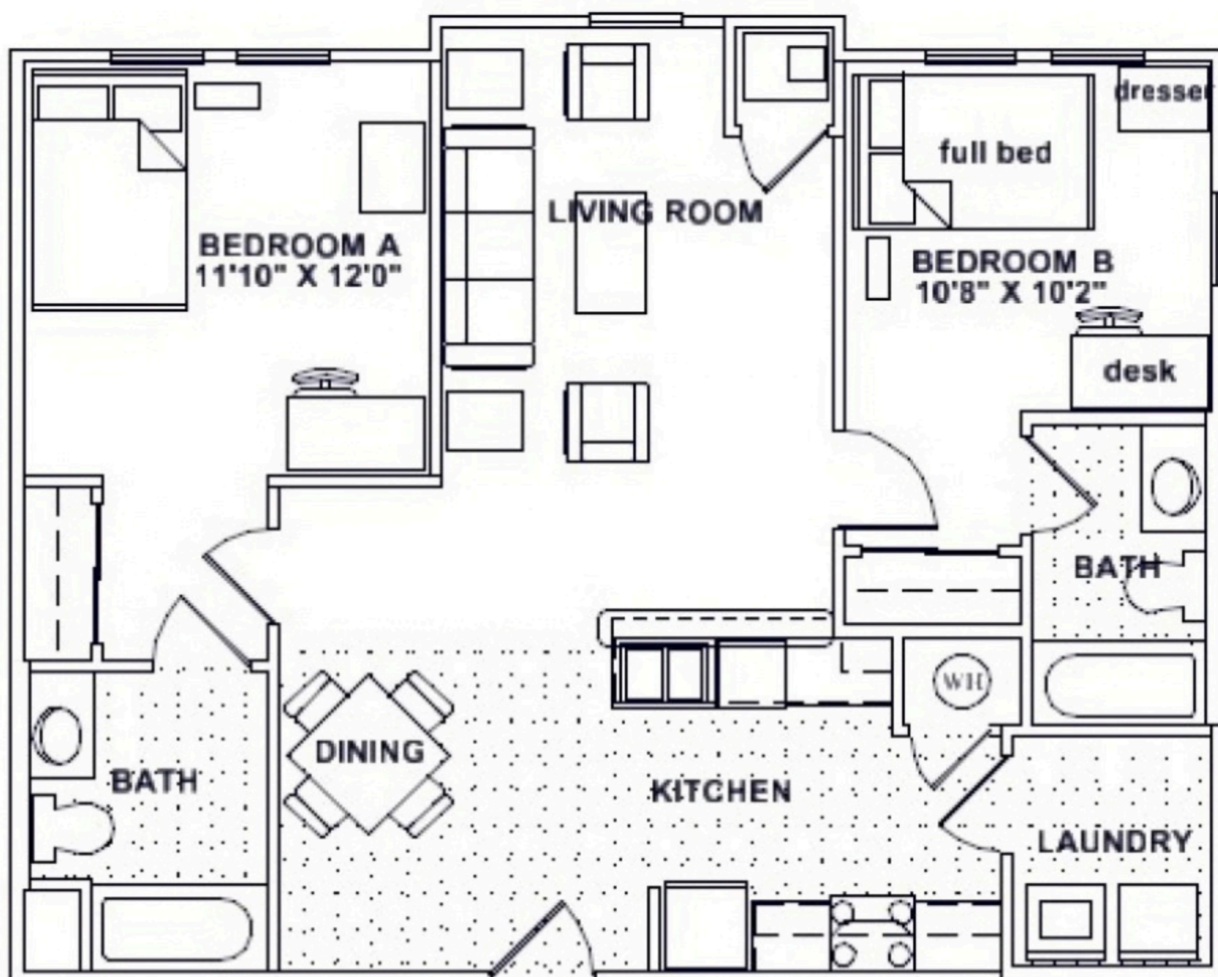
Building 2 and 3 2 bedroom
